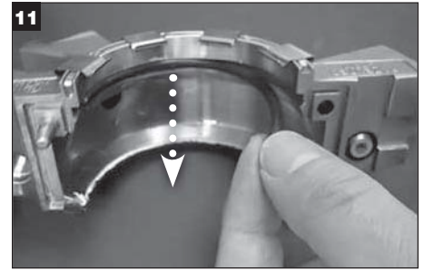
Remove used stationary face O-ring.
