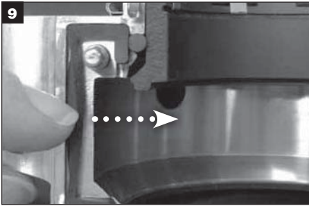
Remove used gland gaskets from gland grooves.
