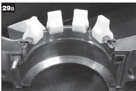
Spring lifter clips installed in gland halves.
