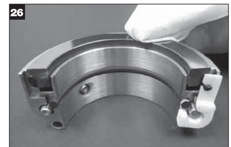
Clean rotary face halves with cleaning wipe.
