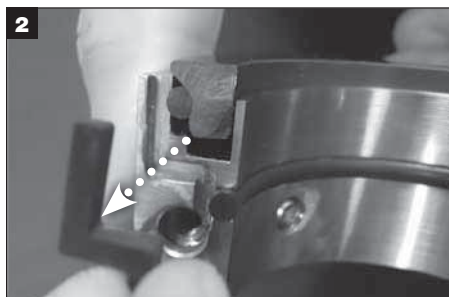
2 Remove used rotary holder gaskets.
