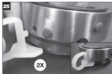
Install installation spacers on OD of holder halves.
