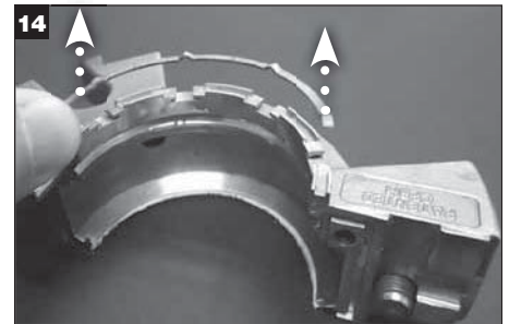
Remove spring lifter halves from gland halves.
