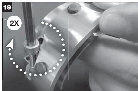
Lubricate threads with a recommended anti seize compound and install holder cap screws in rotary holder half.
