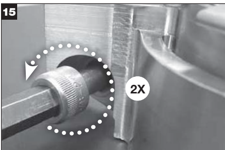
Remove used gland cap screws.
