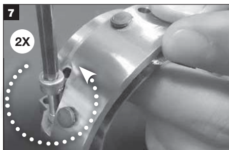
7 Remove used holder cap screws from holder halves.
