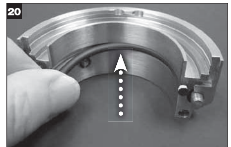
Apply a thin film of grease and install shaft O-ring halves in rotary holder halves. O-rings must protrude evenly from both holder half ends. (Ref. CAD image on page 8).
