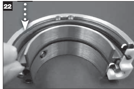
Apply a thin film of grease and install rotary face O-ring halves in rotary holder halves.
