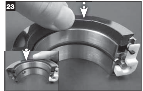
Install rotary face halves in rotary holder halves. Press on face to seat rotary in holder halves.
