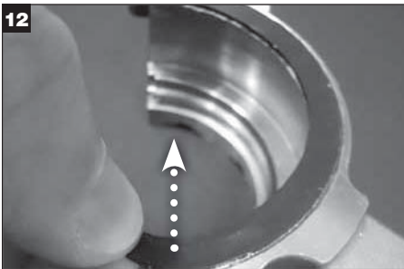
Remove used stuffing box gasket from gland face and all adhesive residue with cleaning solvent
