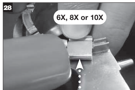
Install springs into spring slots on gland. Use a plastic tipped mallet to ensure springs are seated into place.
