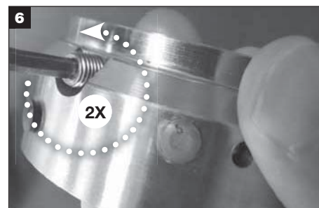
6 Remove used holder set screws (2 places) from rotary holder.
