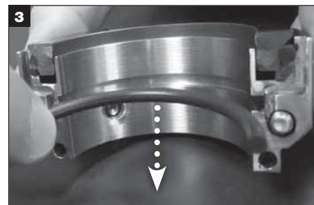
3 Remove used shaft O-ring halves.
