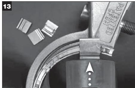
Remove used springs from gland halves by tapping them from the gland half ID with a small hammer
