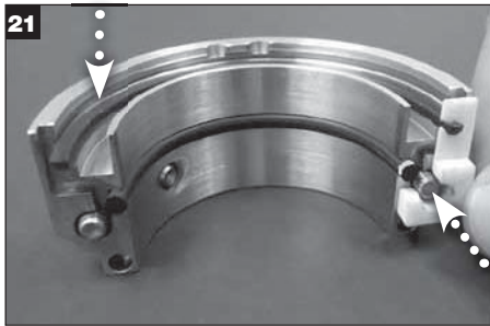
Install rotary holder shipping spacers in rotary holder halves.
