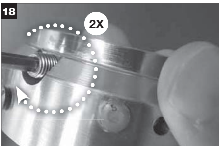
Install new holder set screws (2 places) in rotary holder. IMPORTANT: Prior to installing the rotary holder on the shaft/sleeve, check to ensure the holder set screws are not protruding beyond the inside surface of the rotary holder.
