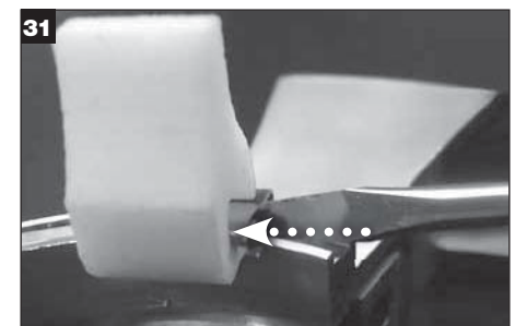
Set spring lifter location using a flat head screwdriver. IMPORTANT: End of spring lifter must be aligned with edge of the end spring. Remove all clips and retain for re-setting lifter location.
