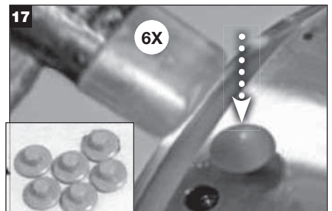
Install new centering buttons on OD of rotary holder. Important: Make sure buttons are fully seated without deforming the exposed heads
